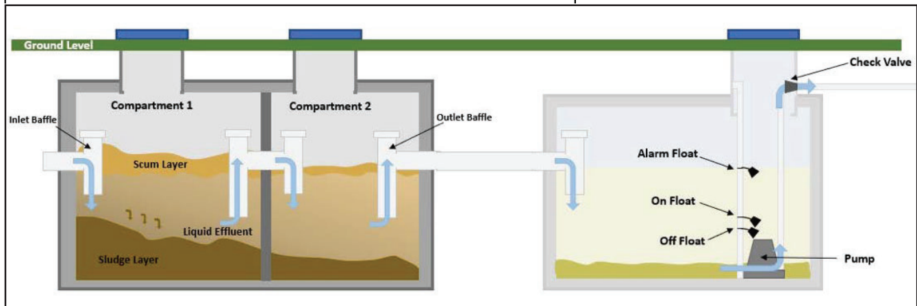
This diagram shows the contents of a pressure distribution septic tank and pump tank.
